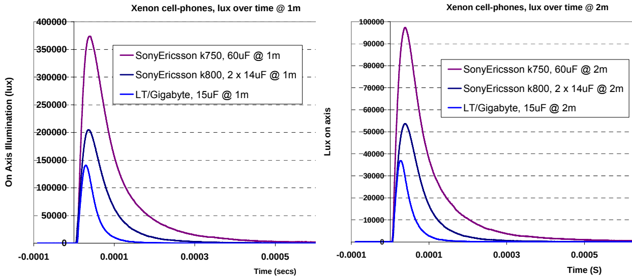
Fig 5: Light power over time for 3 different xenon sources
