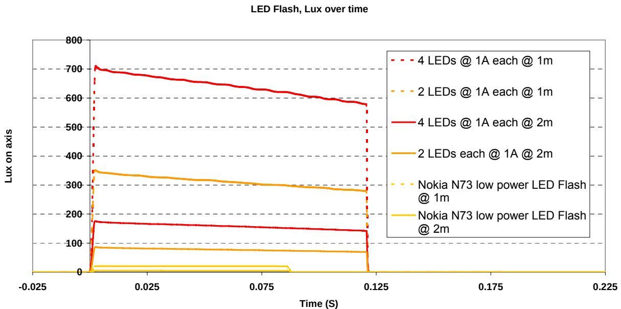
Fig 6: Light power over time for LED Flash
